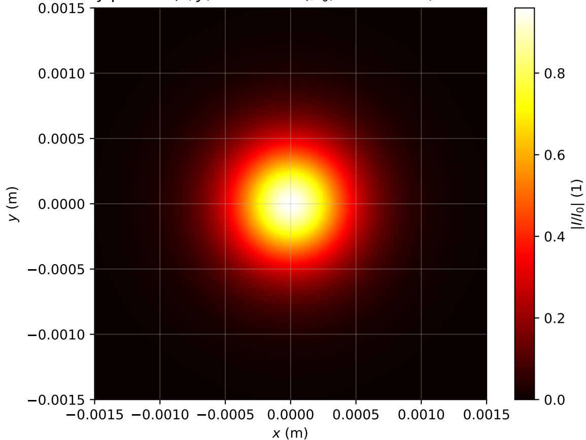
Intensity profile I(x, y, z = 3.582m)/I_0 , P_{in}=0.8P_{cr} , artificial time
